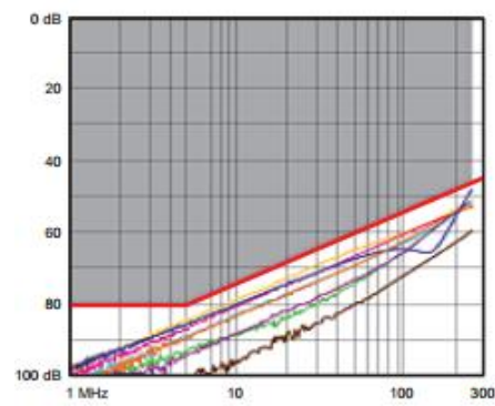
NEXT
