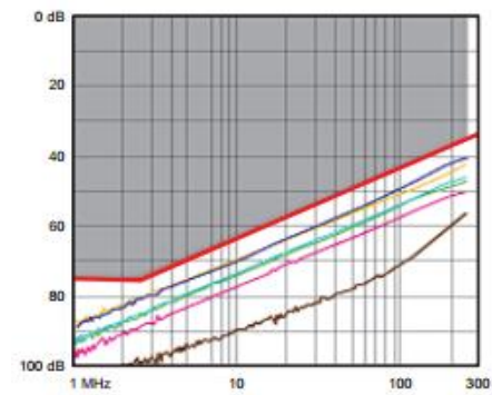
FEXT
