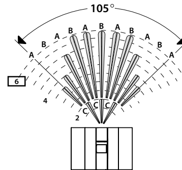
Vista superior K4431
